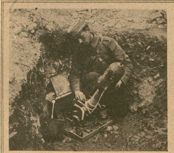
FIRING A FRENCH AIR-TORPEDO: A 58-MM. TRENCH-GUN WITH ITS "FINNED" PROJECTILE IN POSITION.
